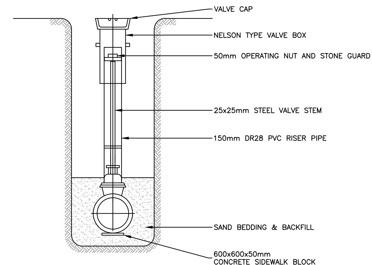
TYPICAL GATE VALVE (SECTION)
