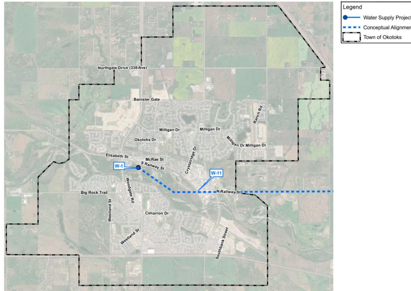
Figure 2: Future Water Supply and Treatment Projects
