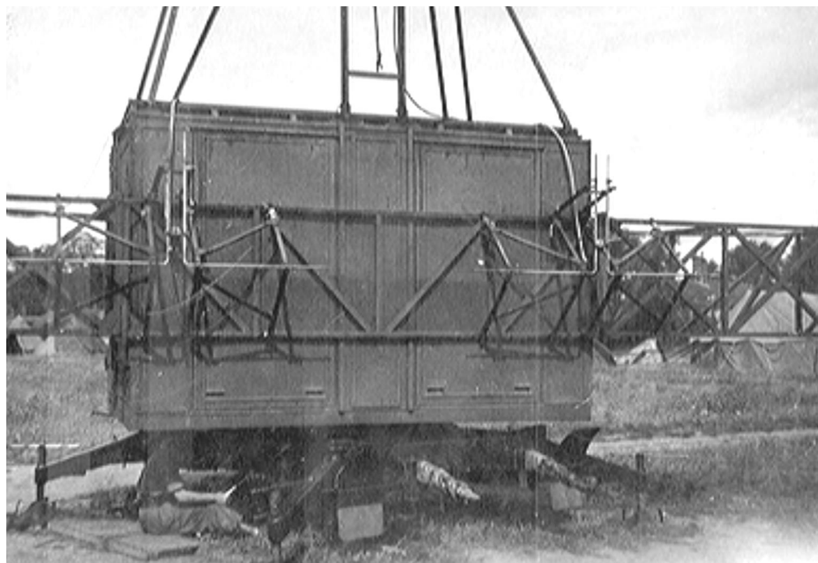
Mortar-detecting radar
